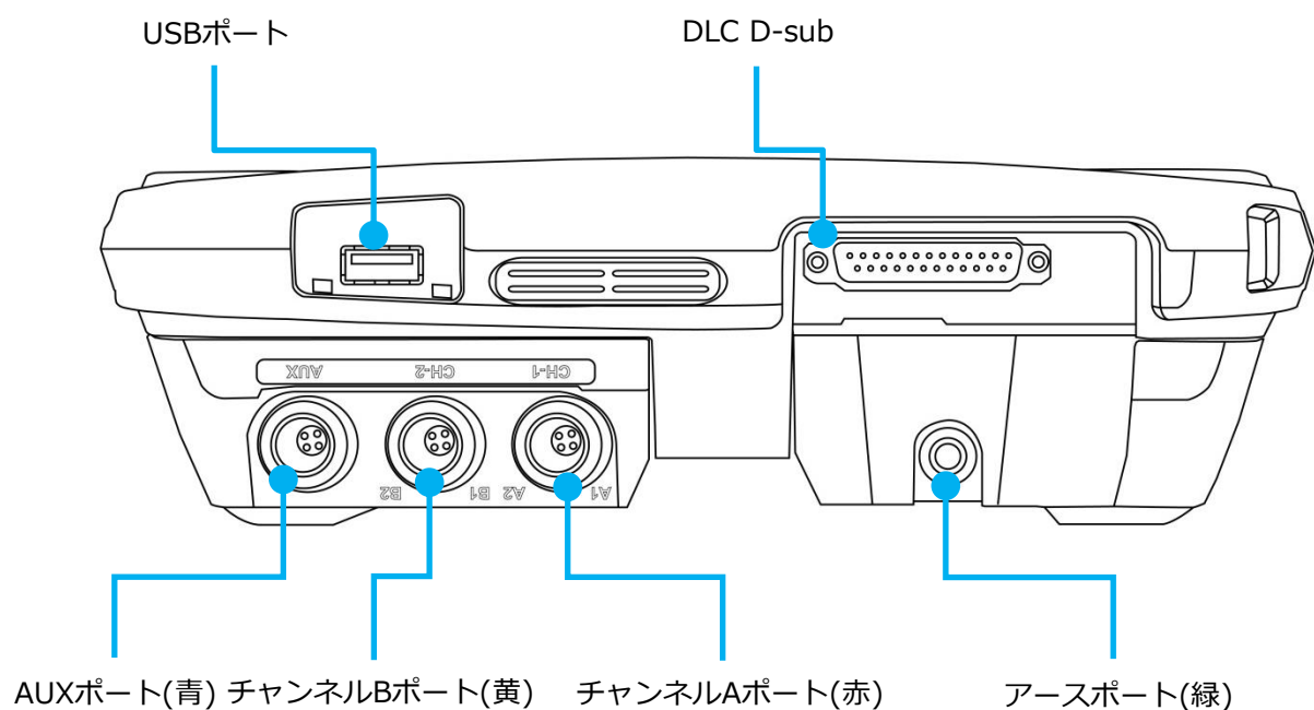
[G-scan2本体上面図]
